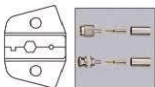
RG-8401 AT & T/ST OR SMA FIBER- OPTIC CONN. 0.190 (4.83MM) HEX, 0.090 (2.29MM) ROUND, 0.105 (2.67MM) ROUND
