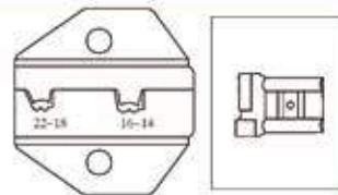
HD-NF 1 FOR NON-INSULATED FLAG TERMINALS FROM 0.5 TO 2.5 SQ. MM. AWG 22-18, 16-14
